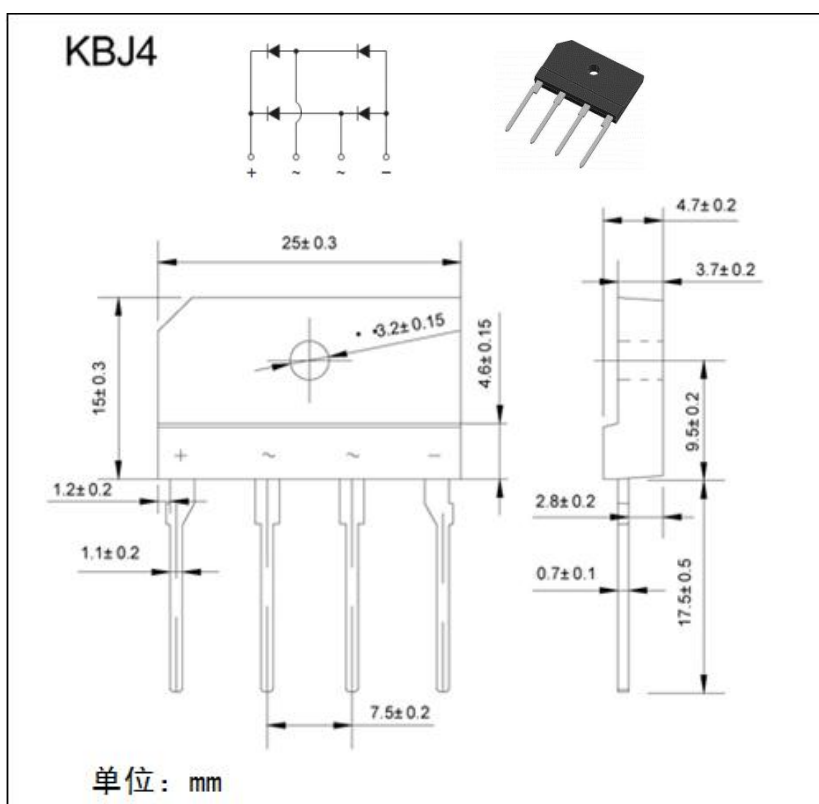
KBJ4 封装外形图：
