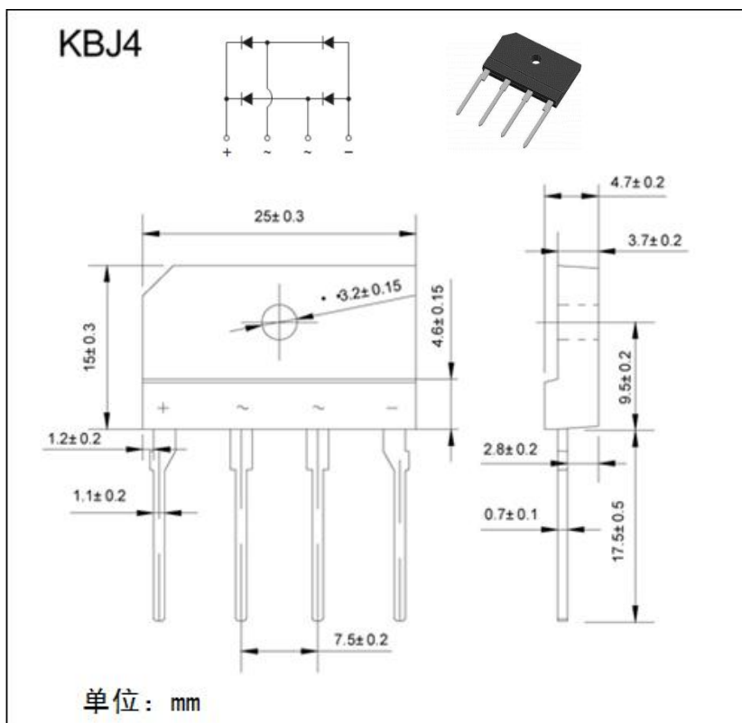
KBJ4 封装外形图:
